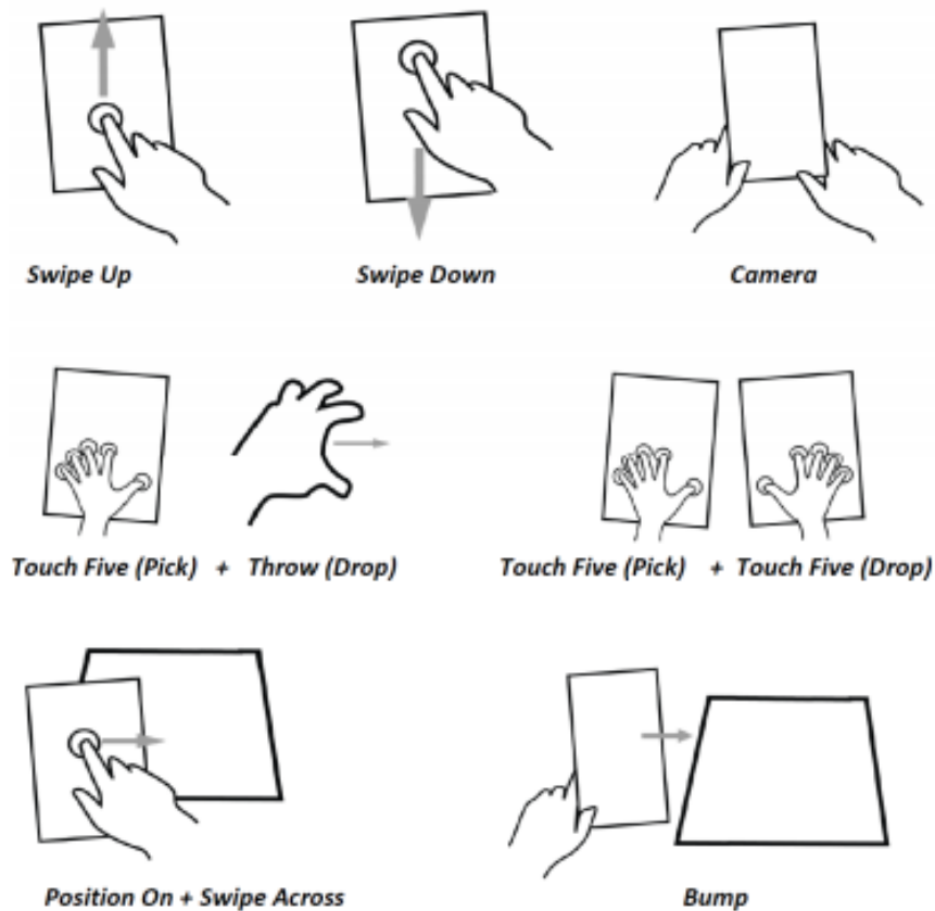
Figure 3: Proposed Gestures from Elicitation Study [9]
